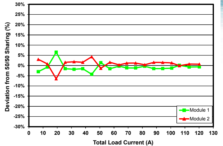
Figure I: Typical current share performance of 2 paralleled modules
